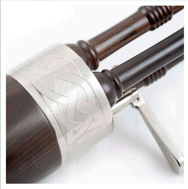
BB/SPA4/M Celtic-engraved ferrule and common stock with drone switch
